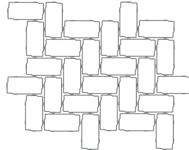
Cluster Pattern Step 2 - Full Stones in herringbone pattern with 1½ stones removed (false joints not shown)
