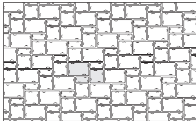
Pattern 11 New 33 sf Squares • 17 sf Sm. Rectangles 50 sf Lg. Rectangles
