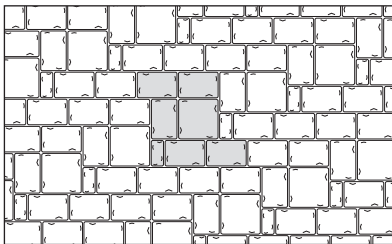
GS Pattern 7 22 sf Grand Squares 73 sf Lg. Rectangles 5 sf Sm. Rectangles
