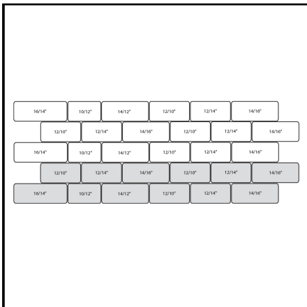
6" High Running Bond 2
