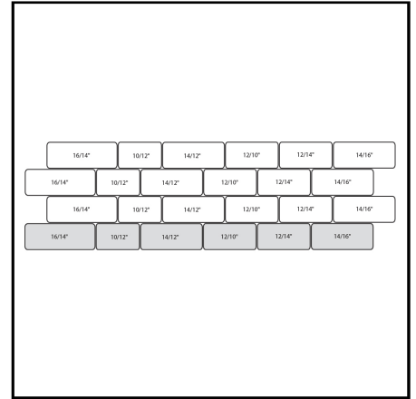
6" High Running Bond 1
