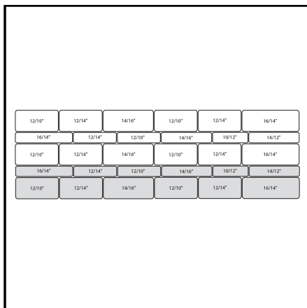
3" & 6" High Running Bond Alternate Rows
