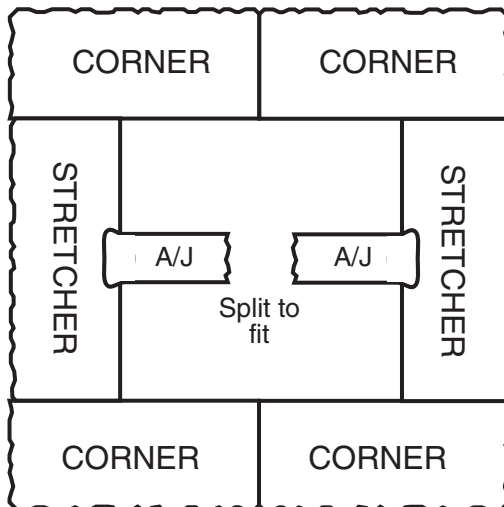
30" x 30" Pillar Alternating Courses
