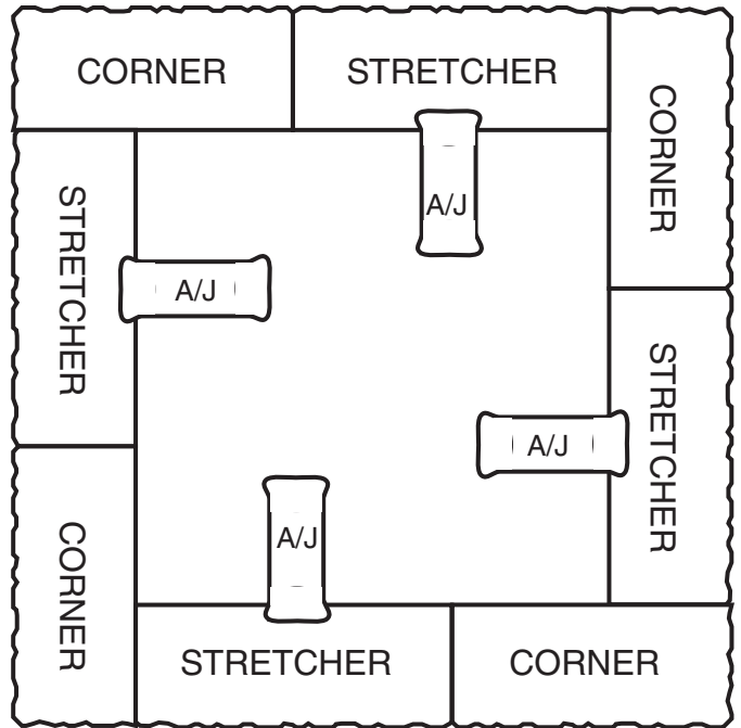
39" x 39" Pillar Alternating Courses
