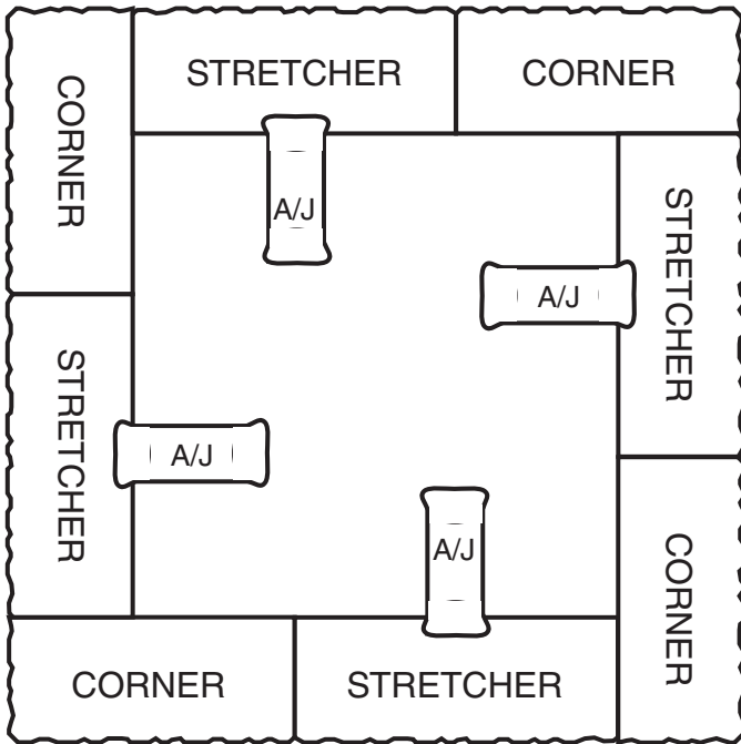
39" x 39" Pillar Alternating Courses
