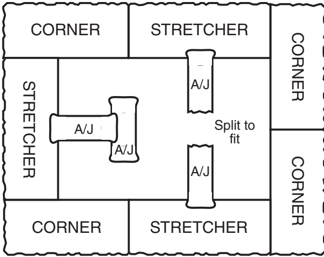
30" x 39" Pillar Alternating Courses
